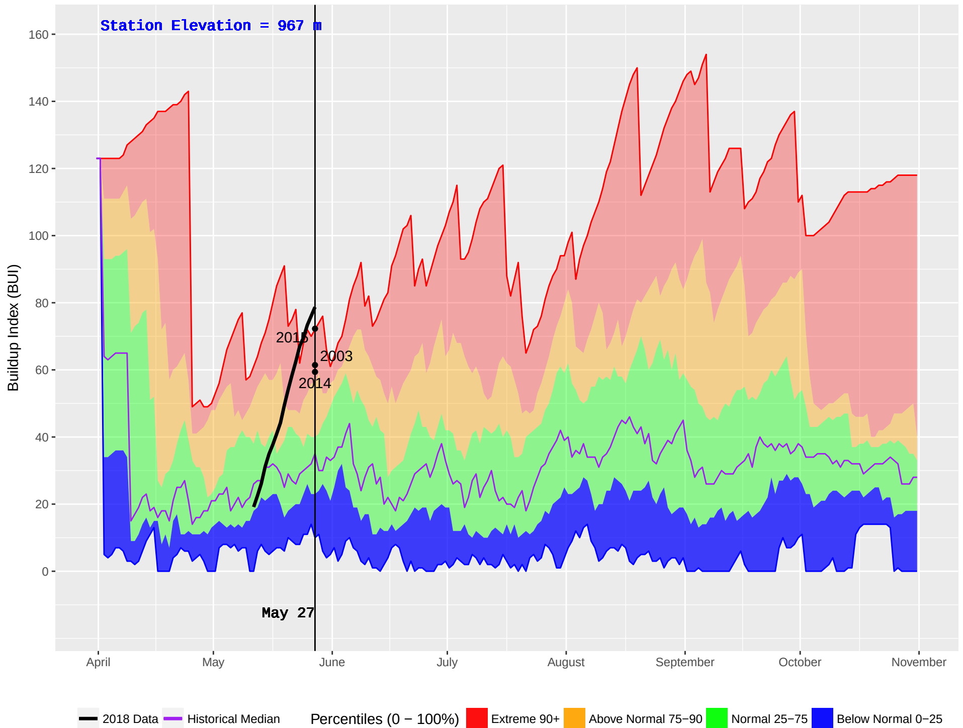
WONOWON (136) : Historical (1990–2016) and Current (2018) Noon Buildup Index (BUI)
