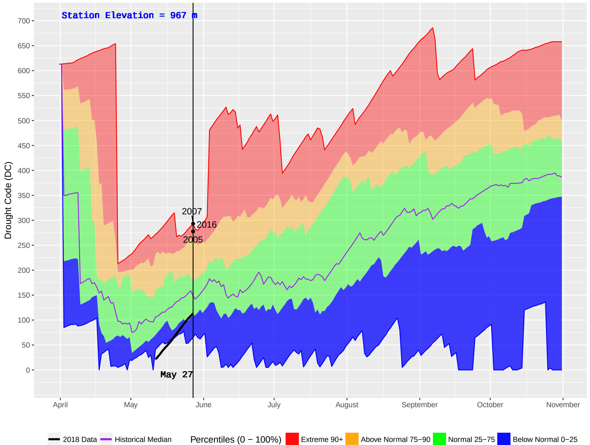
WONOWON (136) : Historical (1990–2016) and Current (2018) Noon Drought Code (DC)
