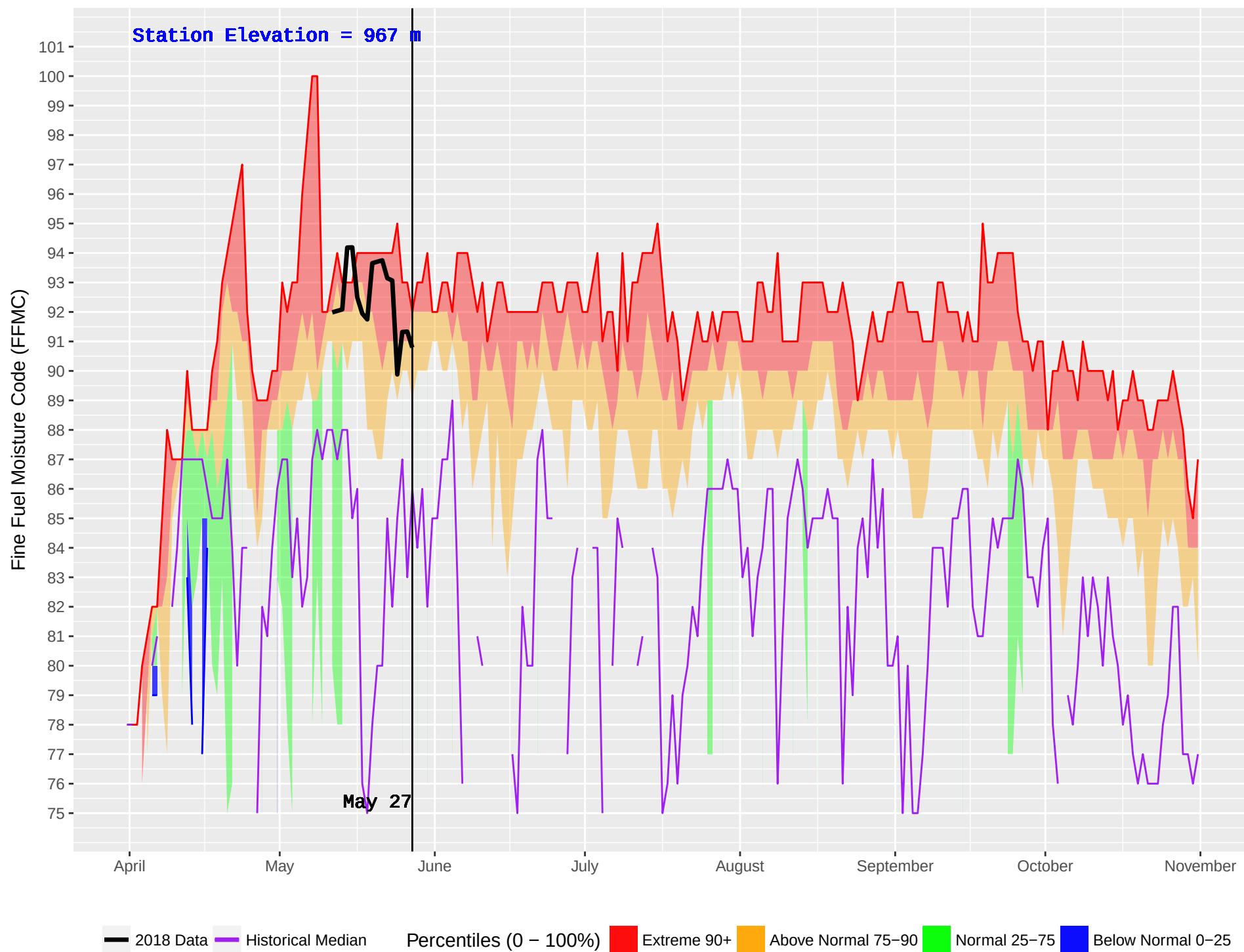
WONOWON (136) : Historical (1990–2016) and Current (2018) Noon Fine Fuel Moisture Code (FFMC)
