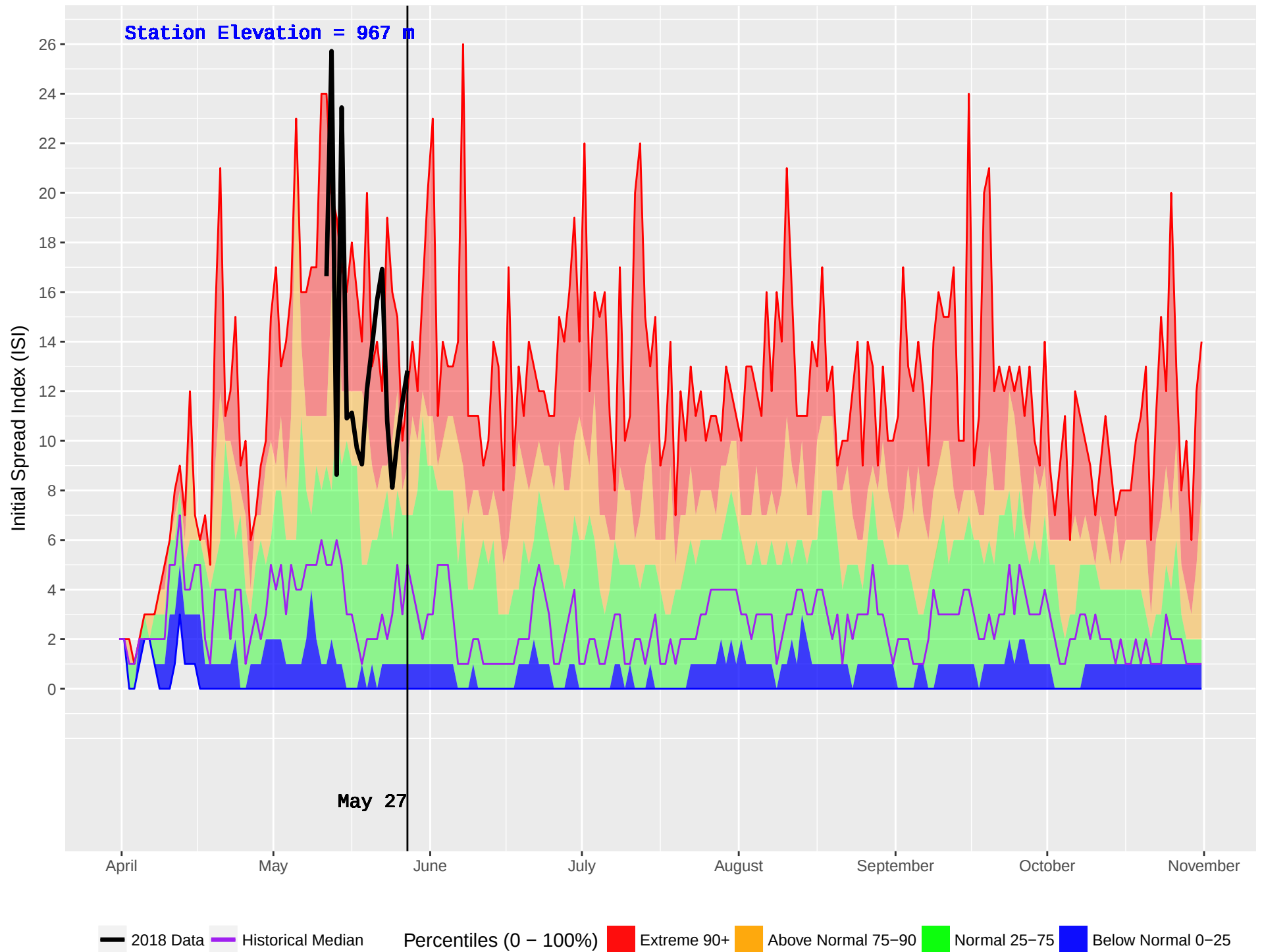
WONOWON (136) : Historical (1990–2016) and Current (2018) Noon Initial Spread Index (ISI)
