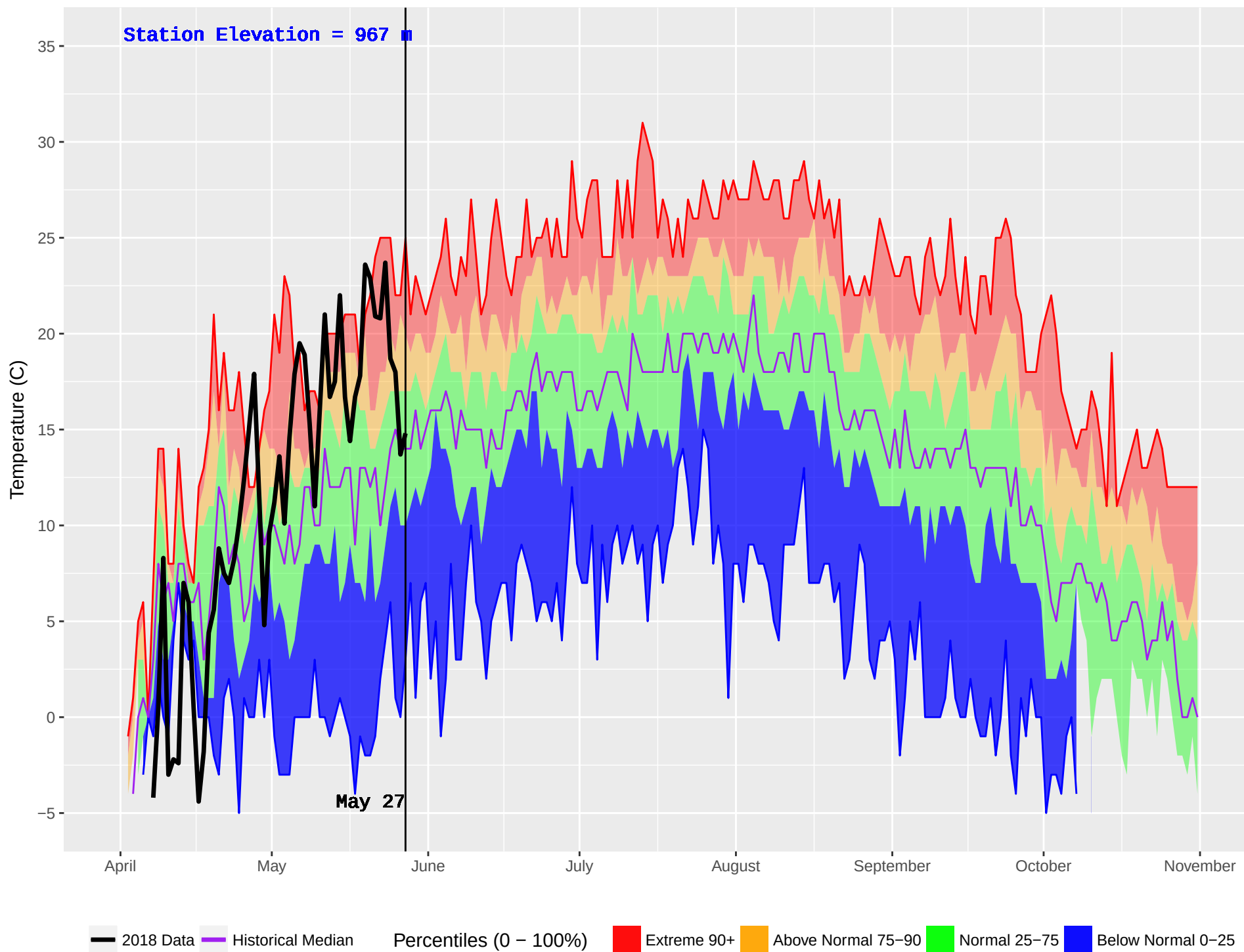
WONOWON (136) : Historical (1990–2016) and Current (2018) Noon Temperature
