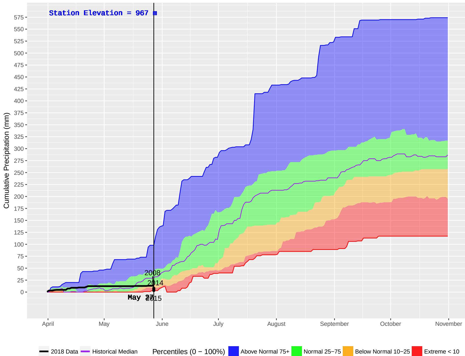
WONOWON (136) : Historical (1990–2016) and Current (2018) Noon Cumulative Precipitation
