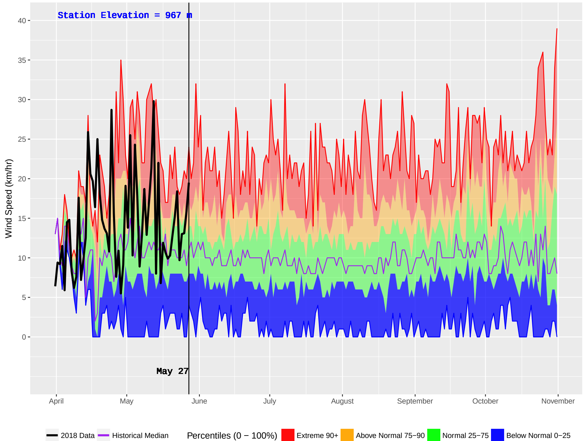
WONOWON (136) : Historical (1990–2016) and Current (2018) Noon Wind Speed
