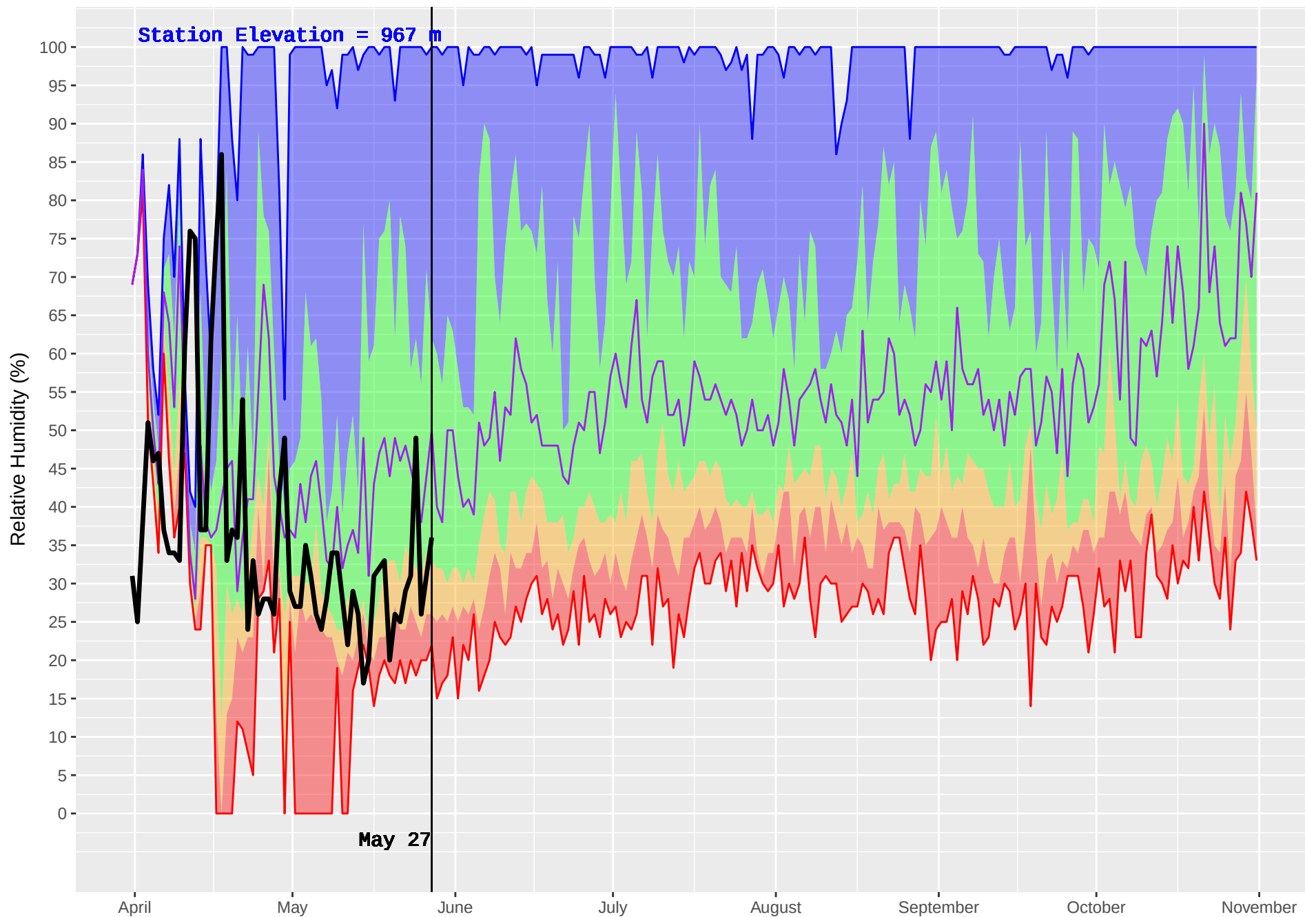
WONOWON (136) : Historical (1990–2016) and Current (2018) Noon Relative Humidity
