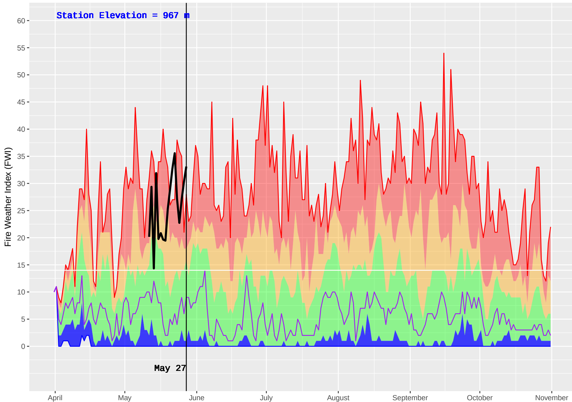
WONOWON (136) : Historical (1990–2016) and Current (2018) Noon Fire Weather Index (FWI)
